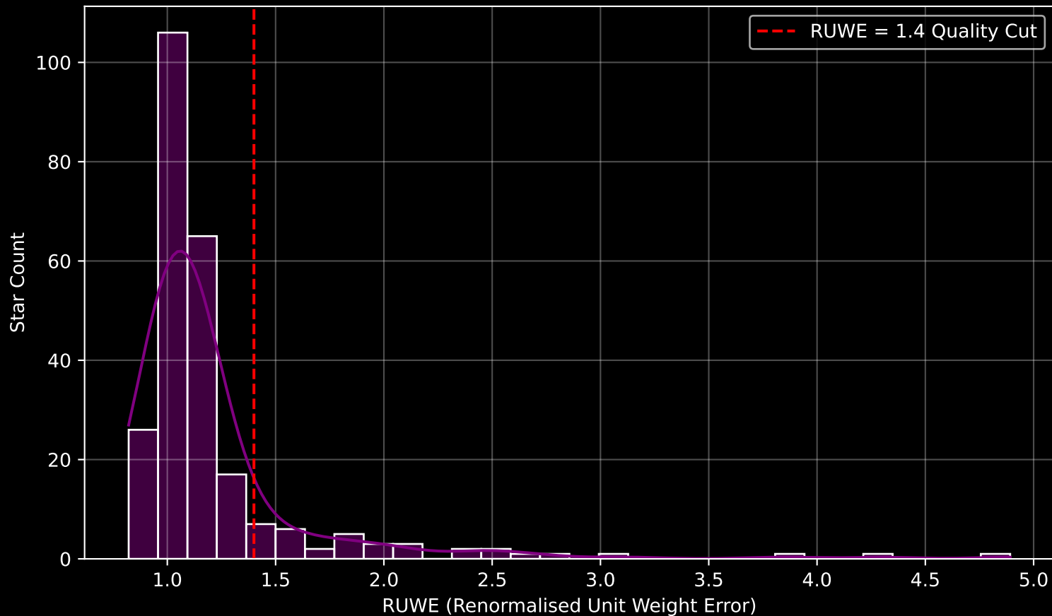
GALAH DR4 Field [211] RUWE Distribution (n= 250)
