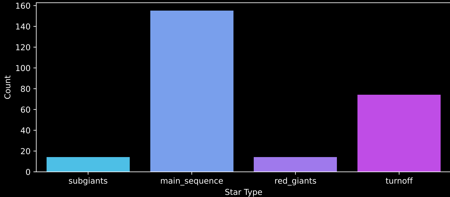
GALAH DR4 Field: [211] Count plot of Star Type
