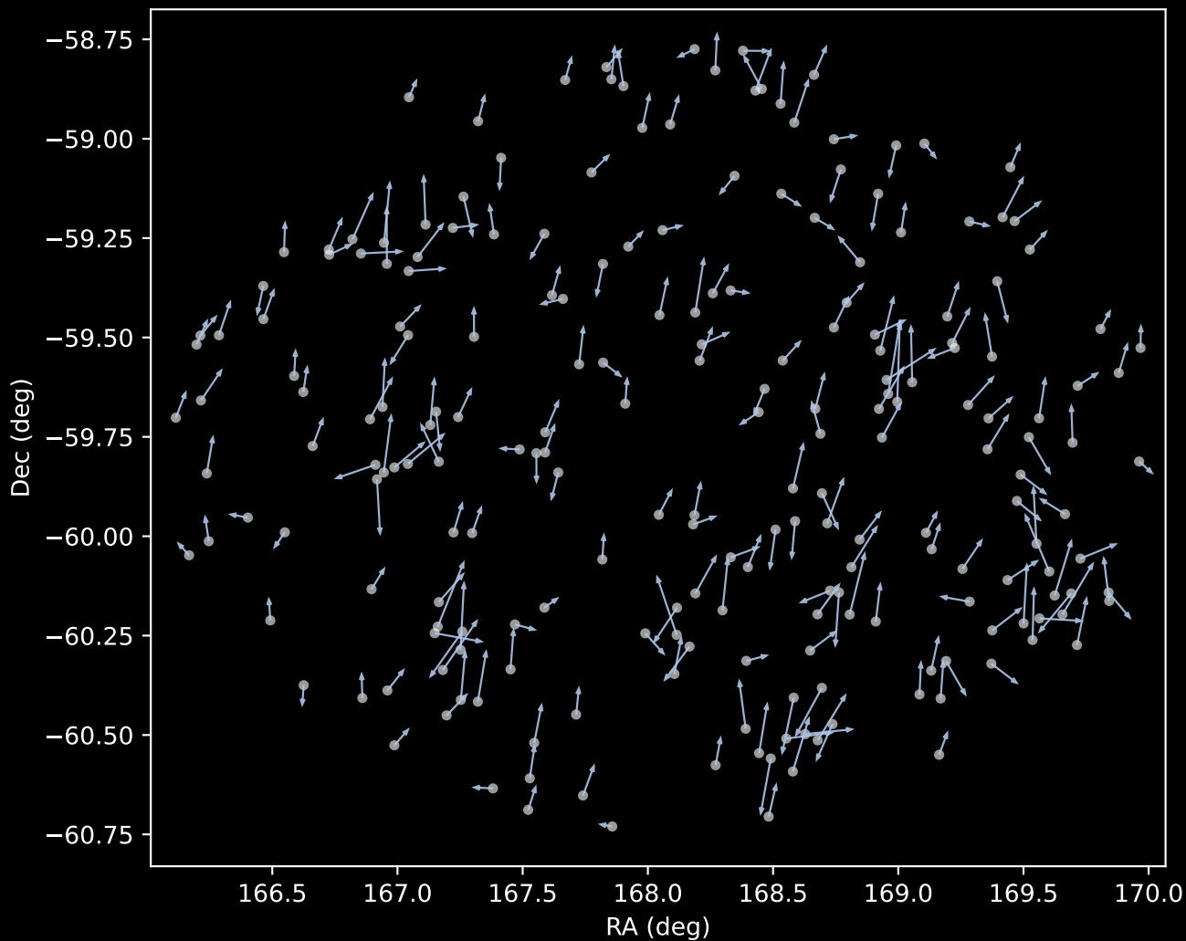
GALAH DR4 Cluster 1 Proper Motion Vectors (n=219)
